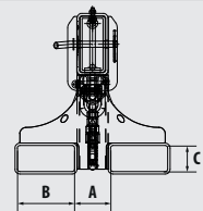
Fork sleeve inside dimensions in mm
